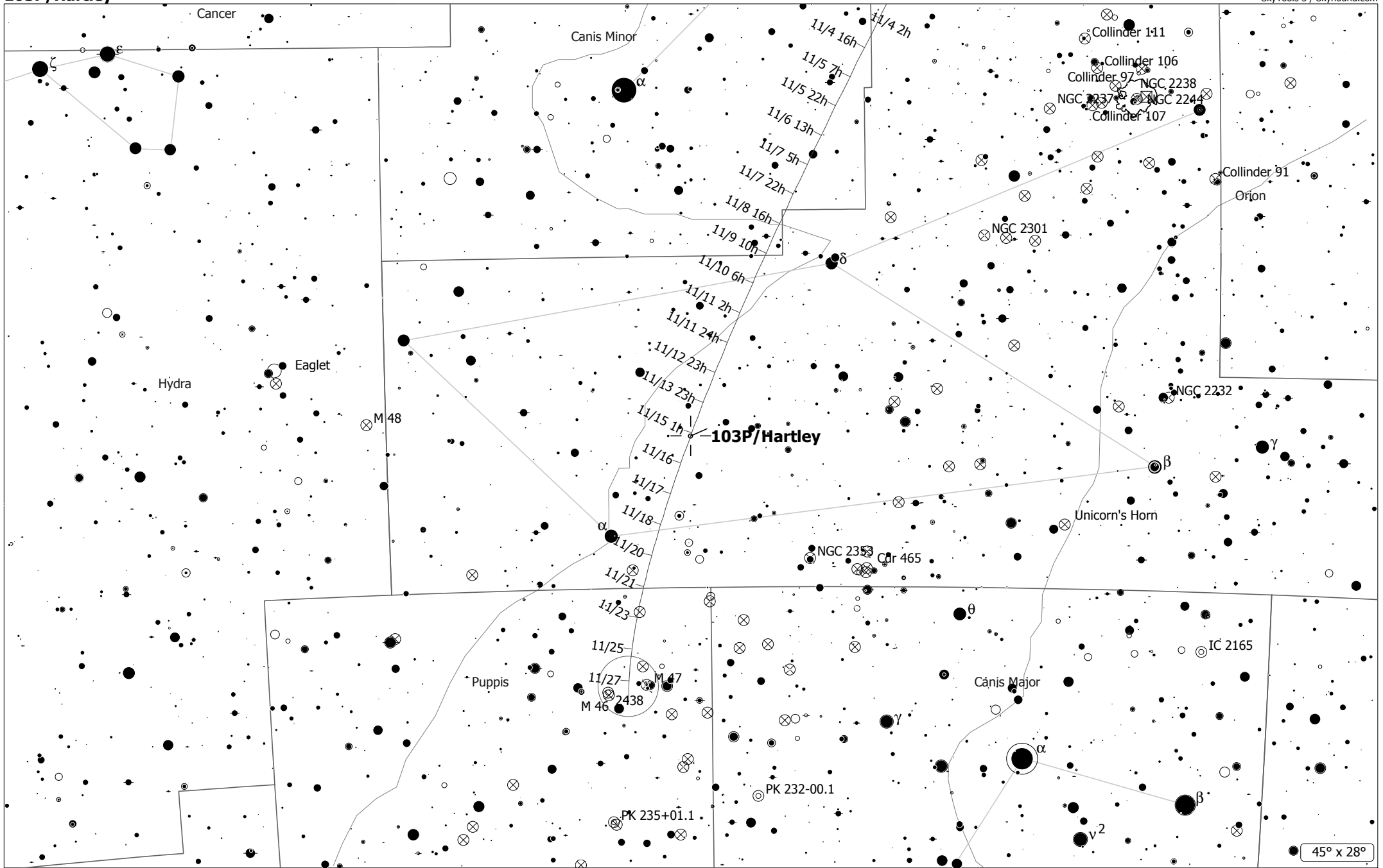
103P/Hartley (Comet)
